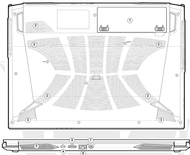
Figure 5 - Bottom & Rear Views
