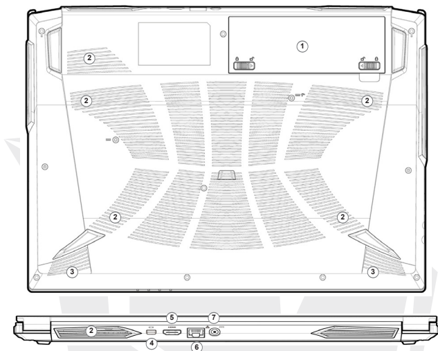
Figure 5 - Bottom & Rear Views
